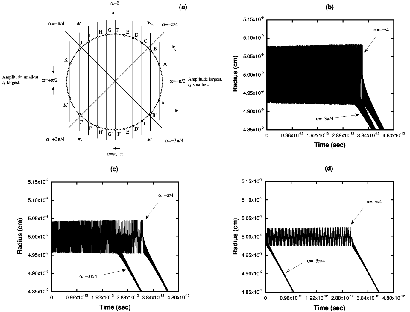
FIG. 5. (a) A schematic figure is shown here to help better illustrate the effect of \alpha on both t_d as well as the amplitude of the spiralling motion, for the situation when A \gg A_c . Each pair of mirror points, such as A and A', B and B', have nearly the same value of t_d for A \gg A_c . Figures 5(b)–5(d) contain plots of r vs t , for a = 0.5 \text{ \AA} . Each plot contains two r vs t curves, one for \alpha = -\pi/4 , and one for the “mirror case” of \alpha = -3\pi/4 . (b) A = 1000 statvolt; (c) A = 300 statvolt; (d) A = 100 statvolt. As can be seen, as A decreases, the behavior between the \alpha = -\pi/4 and \alpha = -3\pi/4 curves becomes increasingly different, in agreement with Fig. 3. For A = 100 statvolt, the \alpha = -3\pi/4 curve is not even stable. Also apparent is the decrease in amplitude of the spiraling motion, and the decrease in t_d as A decreases.
